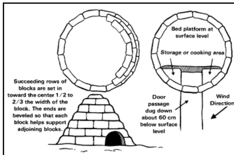
Figure 10-9. Snow house.
