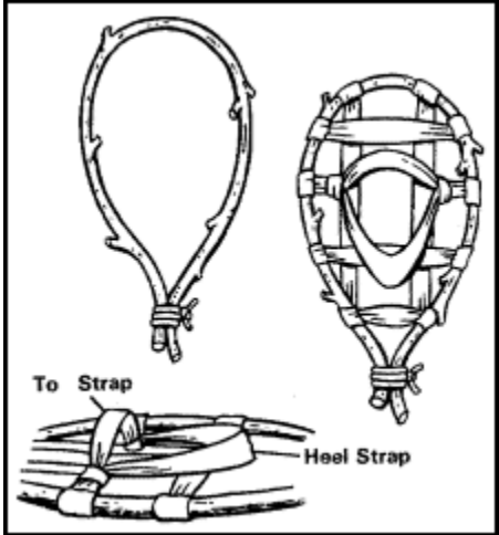
Figure 8-2. Improvised snowshoes.
